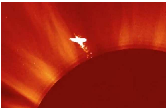
SOHO image of a solar bird-like plasma ejection
